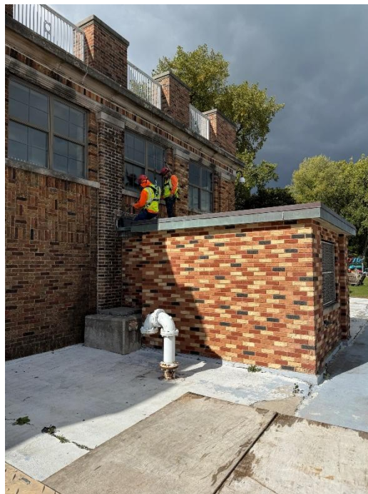
Figure 2: Disconnecting roofing material from main building.
