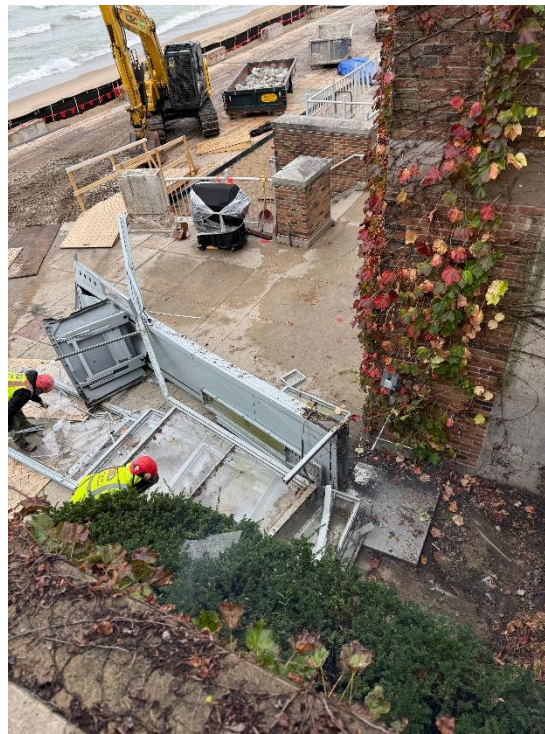
Figure 8: Removal of lower tier ADA lift.
