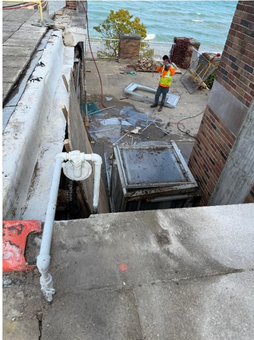
Figure 5: Additional view of demolished ADA lift and concrete on the roof deck.
