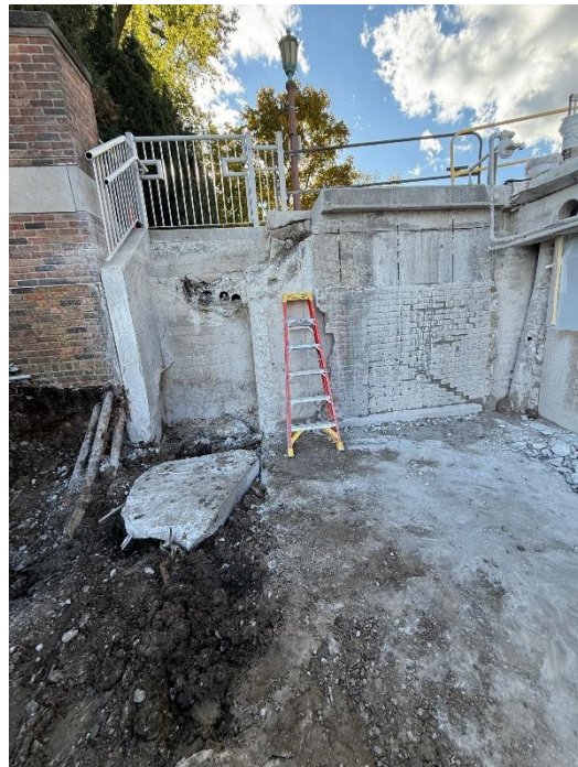
Figure 6: Demolition of southwest corner of the building.
