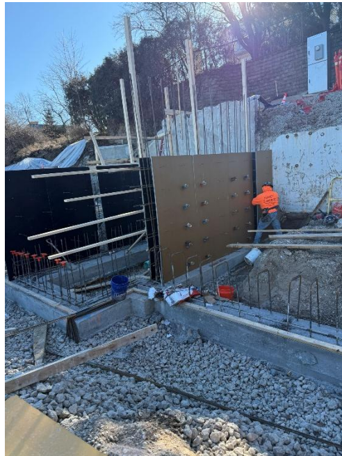
Figure 6: Framing and rebar being installed for new stairs.
