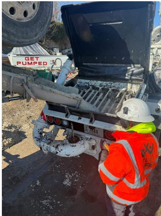
Figure 2: Loading pump truck with concrete.
