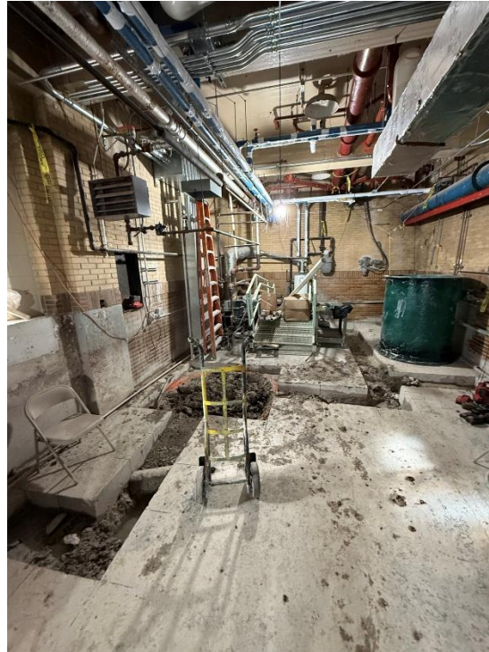
Figure 3: Photo of saw cut concrete floor to accommodate new plumbing rough in.
