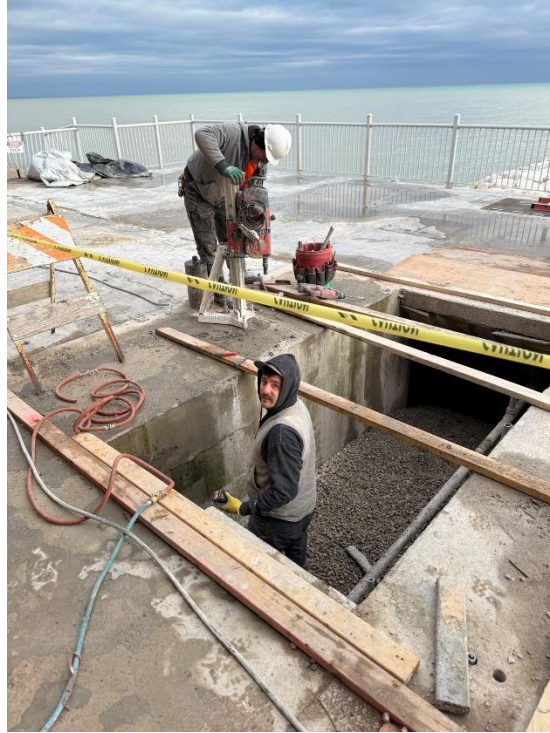
Figure 1: Building area on the east side is being prepared to receive new concrete.
