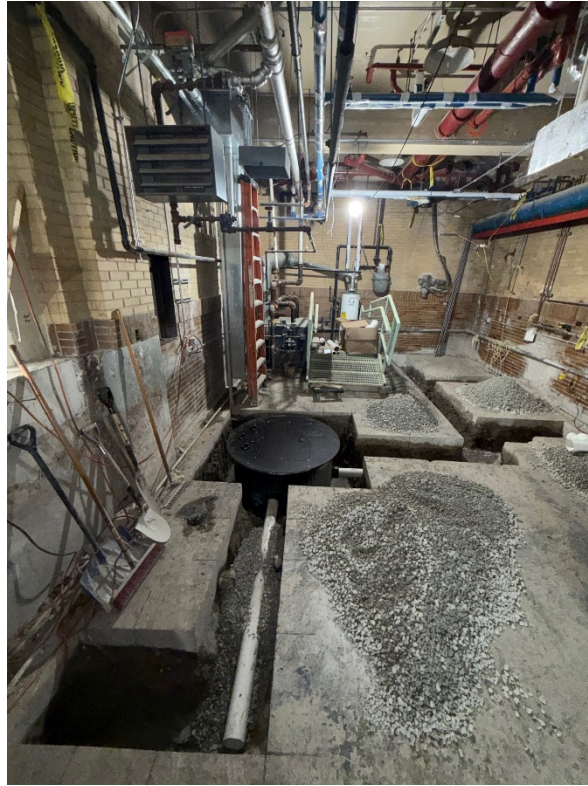
Figure 1: Sewage Ejector Pit Install.
