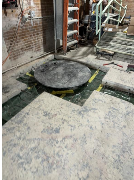
Figure 3: Injector pit backfilled and ready for concrete.
